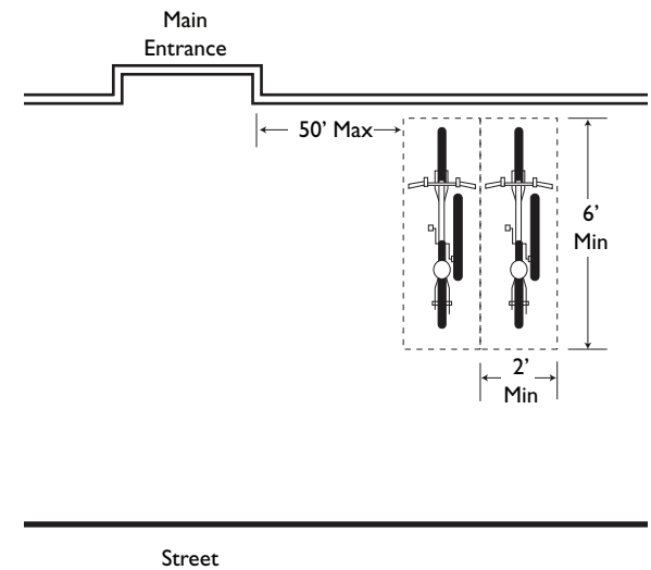
Figure 6-2: Bicycle Parking
